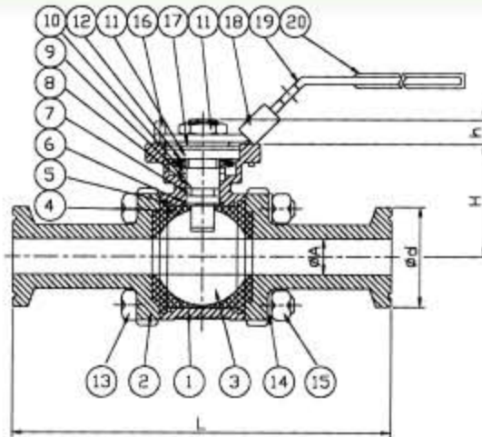
1/2"-3" FULL PORT
